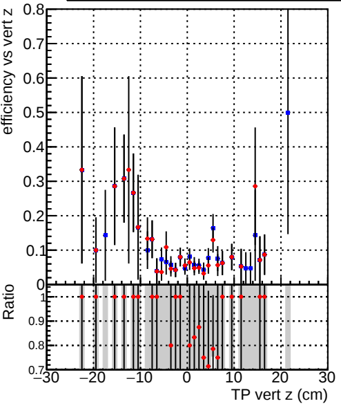
Efficiency vs TP vert z (cm) Legend: DQM_TT_mkFit-DQM_original-lowpt DQM_TT_mkFit-DQM_updated-lowpt
