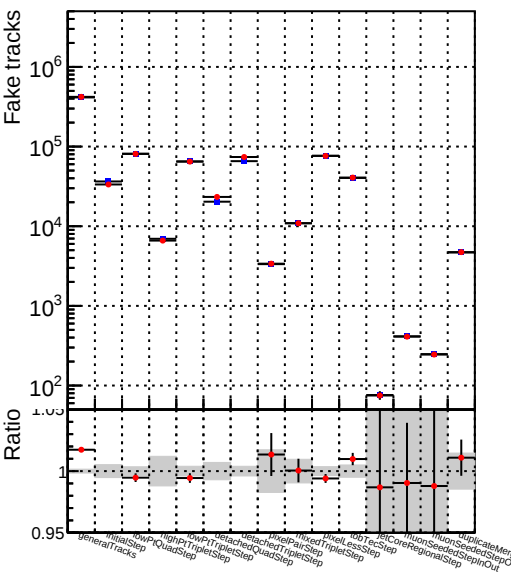
Number —●— DQM_TT__mkFit-DQM_updated-lowpt
