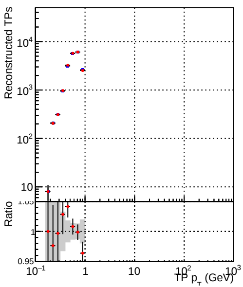
Legend: DQM_TT_mkFit-DQM_original-lowpt (blue line), DQM_TT_mkFit-DQM_updated-lowpt (red line)
