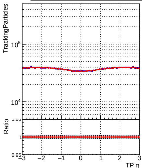
Legend: DQM_TT_mkFit-DQM_original-lowpt (blue line), DQM_TT_mkFit-DQM_updated-lowpt (red line)
