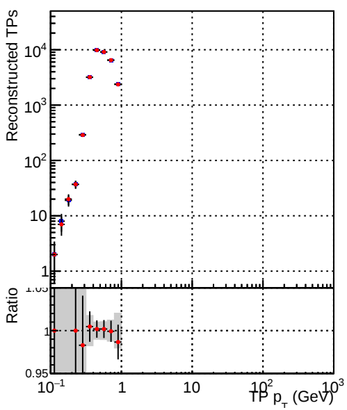
Legend: DQM_TT_mkFit-DQM_original-lowpt (blue line with dots), DQM_TT_mkFit-DQM_updated-lowpt (red line with dots)
