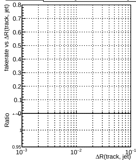
—•— DQM_TT_mkFit-DQM_original-lowpt —•— DQM_TT_mkFit-DQM_updated-lowpt
