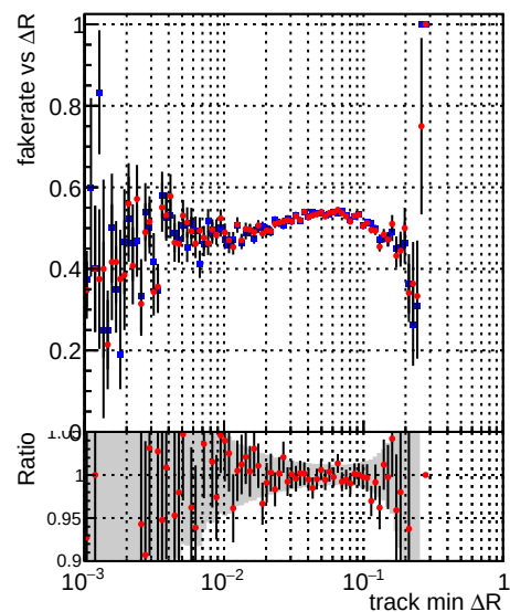
—•— DQM_TT_mkFit-DQM_original-lowpt —•— DQM_TT_mkFit-DQM_updated-lowpt
