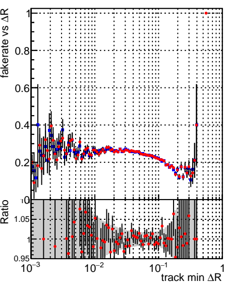
—●— DQM_TT_mkFit-DQM_original-lowpt —●— DQM_TT_mkFit-DQM_updated-lowpt
