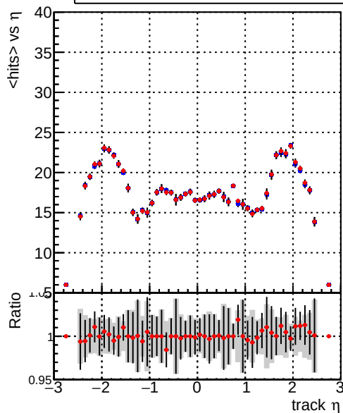
mean hits — DQM_TT_mkFit-DQM_original-lowpt — DQM_TT_mkFit-DQM_updated-lowpt
