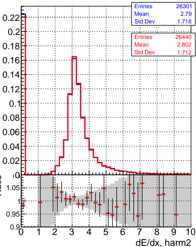
—■— DQM_TT_mkFit-DQM_original-lowpt —●— DQM_TT_mkFit-DQM_updated-lowpt
