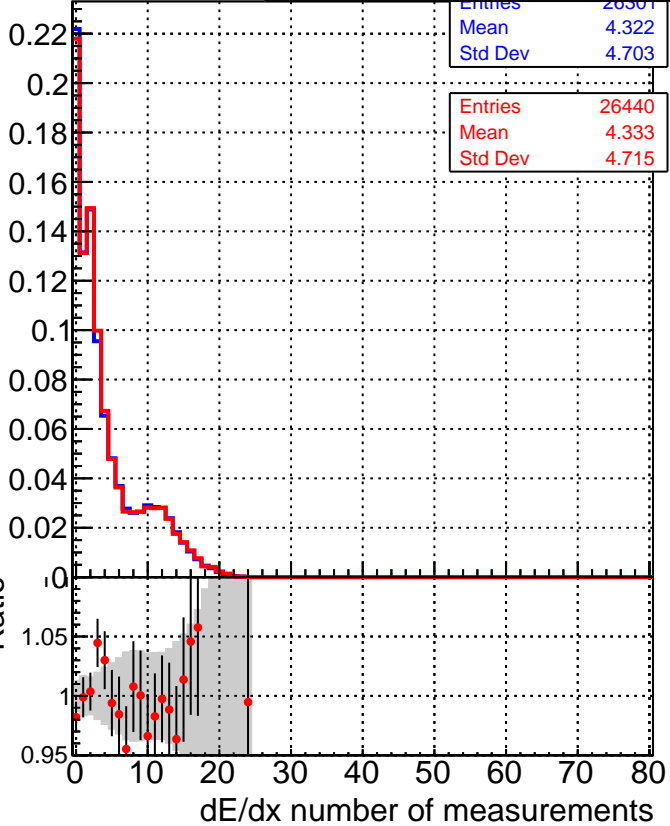
—■— DQM_TT_mkFit-DQM_original-lowpt —●— DQM_TT_mkFit-DQM_updated-lowpt
