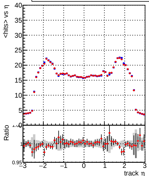
mean hit — DQM_TT_mkFit-DQM_original-lowpt — DQM_TT_mkFit-DQM_updated-lowpt
