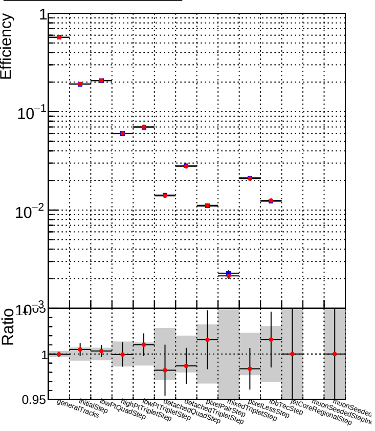
DQM_TT_mkFit-DQM_original-0 DQM_TT_mkFit-DQM_updated-0
