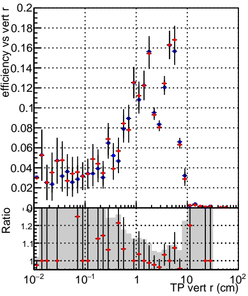
Legend: DQM_TT_mkFit-DQM_original-0 (blue squares), DQM_TT_mkFit-DQM_updated-0 (red circles)
