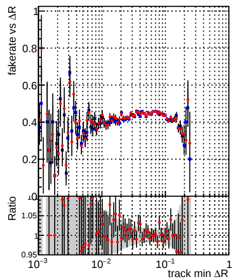
—•— DQM_TT_mkFit-DQM_original-0 —•— DQM_TT_mkFit-DQM_updated-0
