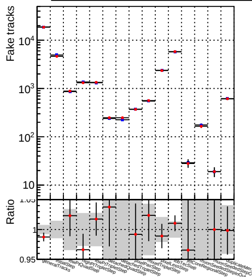
Number —●— DQM_TT_mkFit-DQM_updated-0
