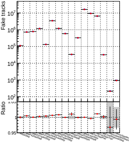
Number —●— DQM_TT_mkFit-DQM_updated-0
