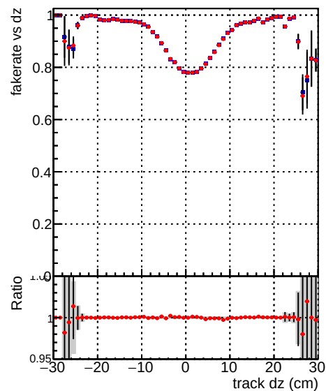
Fake rate vs dz —●— DQM TT mkFit-DQM_original-0 —●— DQM TT mkFit-DQM_updated-0
