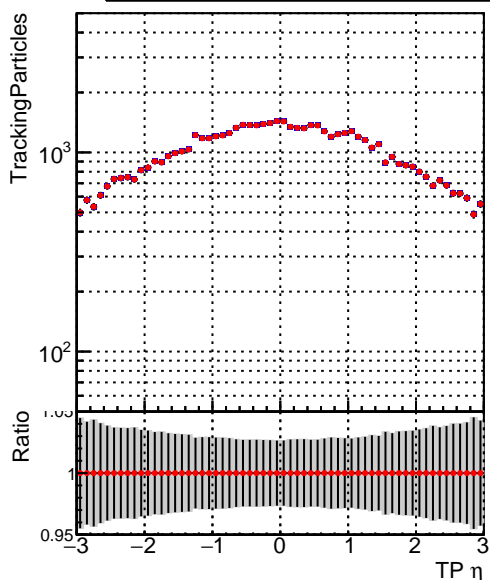
■ DQM_TT_mkFit-DQM_original-0 ● DQM_TT_mkFit-DQM_updated-0
