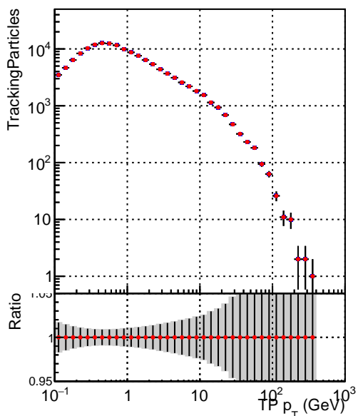
■ DQM_TT_mkFit-DQM_original-0 ● DQM_TT_mkFit-DQM_updated-0
