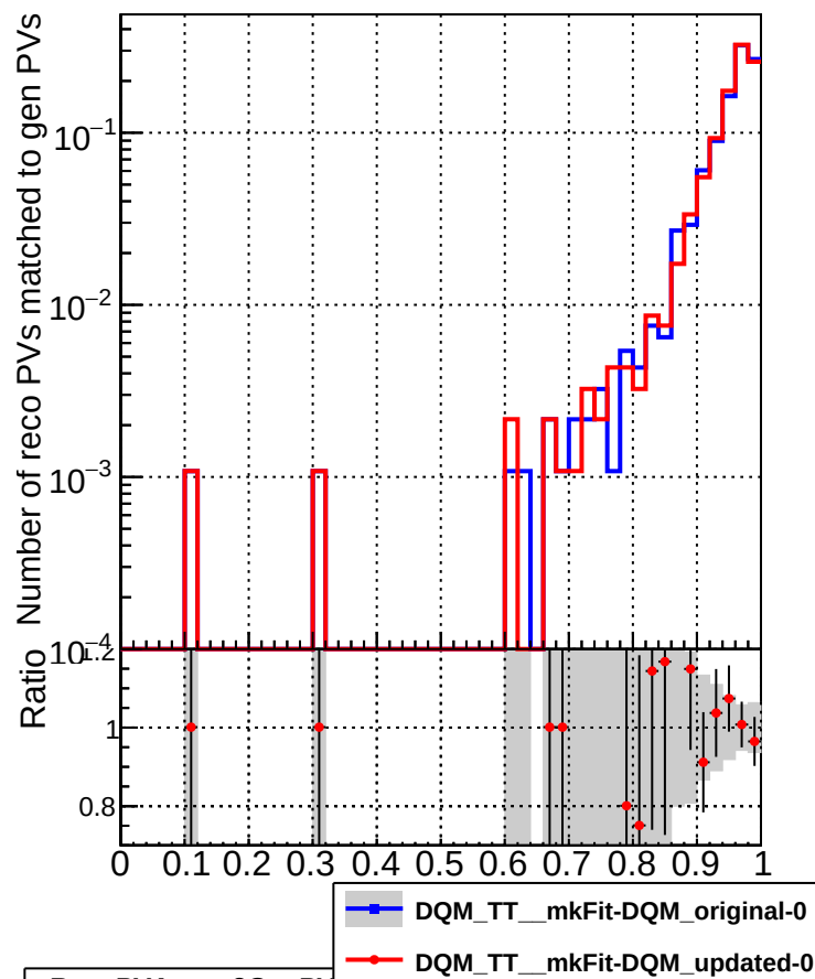
RecoPVAssoc2GenPVmatched_missing
