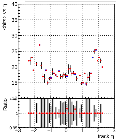
mean hit — DQM_TT_mkFit-DQM_original-0 — DQM_TT_mkFit-DQM_updated-0
