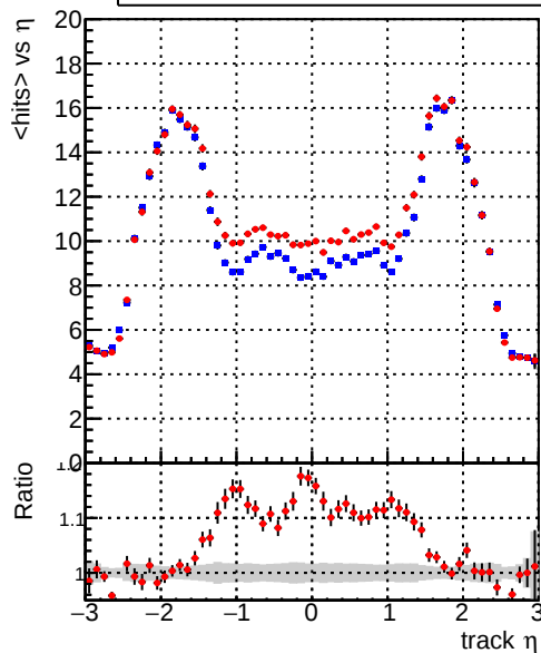
Legend: — DQM_TT_mkFit-DQM_original-0 — DQM_TT_mkFit-DQM_updated-0 mean hits
