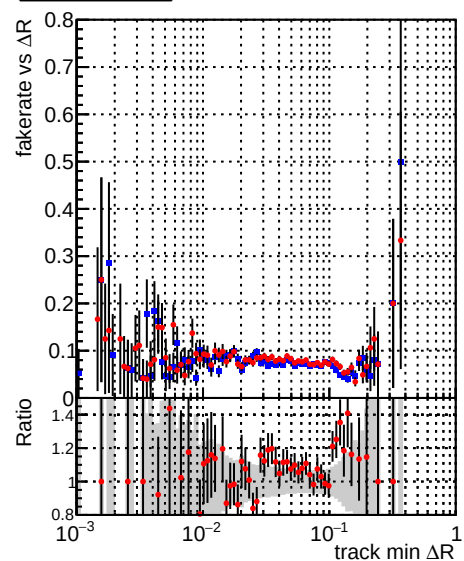
—•— DQM_TT_mkFit-DQM_original-0 —•— DQM_TT_mkFit-DQM_updated-0
