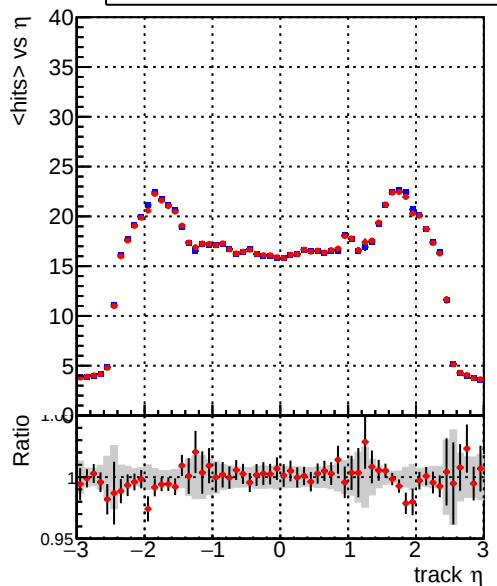
mean hit — DQM_TT_mkFit-DQM_original-0 — DQM_TT_mkFit-DQM_updated-0
