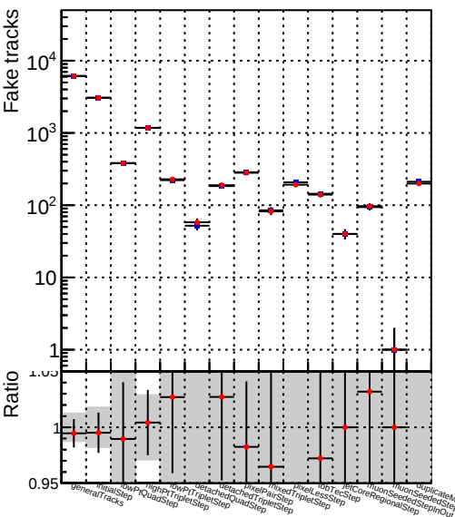
Number —●— DQM_TT__mkFit-DQM_updated-0
