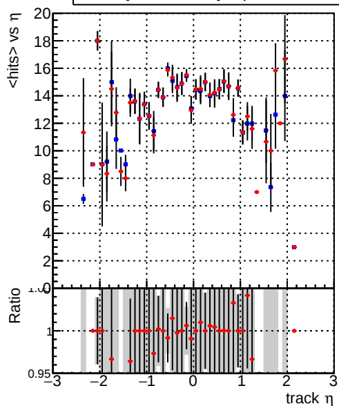
— DQM_TT_mkFit-DQM_original-0 — DQM_TT_mkFit-DQM_updated-0
