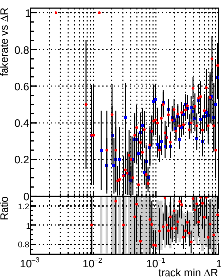
DQM_TT_mkFit-DQM_original-0 DQM_TT_mkFit-DQM_updated-0
