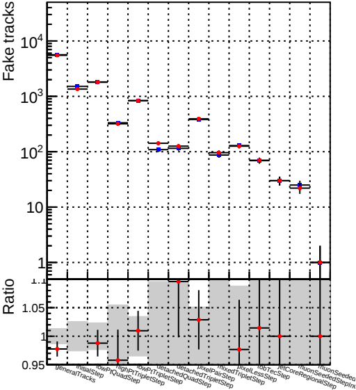
Number —●— DQM_TT_mkFit-DQM_updated-0
