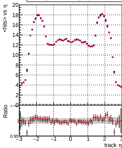
mean hit — DQM_TT_mkFit-DQM_original-0 — DQM_TT_mkFit-DQM_updated-0
