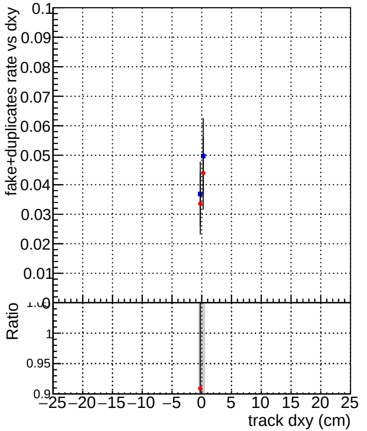
DQM_TT_mkFit-DQM_original-0 DQM_TT_mkFit-DQM_updated-0
