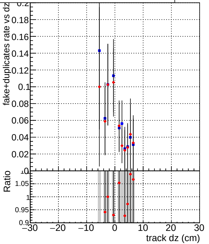
DQM_TT_mkFit-DQM_original-0 DQM_TT_mkFit-DQM_updated-0
