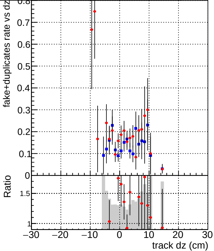
DQM_TT_mkFit-DQM_original-0 DQM_TT_mkFit-DQM_updated-0
