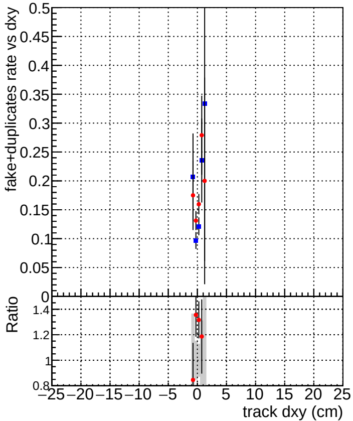
DQM_TT_mkFit-DQM_original-0 DQM_TT_mkFit-DQM_updated-0
