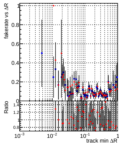
—■— DQM_TT_mkFit-DQM_original-0 —●— DQM_TT_mkFit-DQM_updated-0
