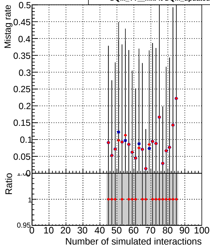
■ DQM_TT_mkFit-DQM_original-0 ● DQM_TT_mkFit-DQM_updated-0
