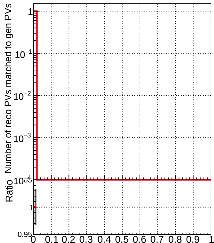
RecoPVAssoc2GenPVMatched_Purity
