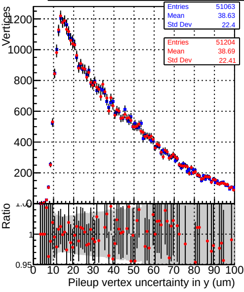
Legend: DQM_TT_mkFit-DQM_original-0 (blue line with dots), DQM_TT_mkFit-DQM_updated-0 (red line with dots)
