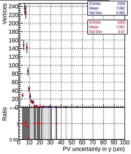
Legend: DQM_TT_mkFit-DQM_original-0 (blue line with dots), DQM_TT_mkFit-DQM_updated-0 (red line with dots)
