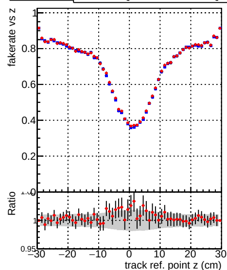
■ DQM_TT_mkFit-DQM_original-0 ● DQM_TT_mkFit-DQM_updated-0
