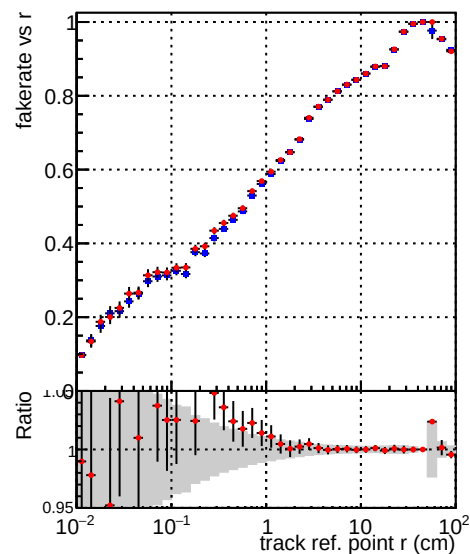
■ DQM_TT_mkFit-DQM_original-0 ● DQM_TT_mkFit-DQM_updated-0
