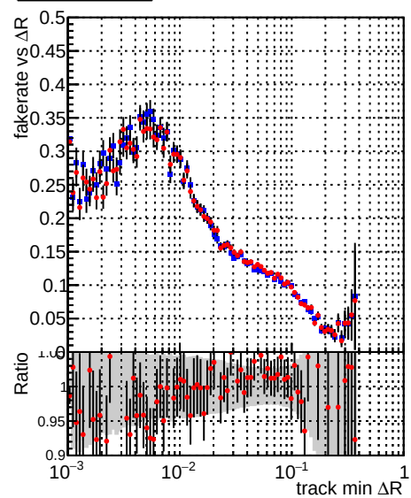
—•— DQM_TT_mkFit-DQM_original-0 —•— DQM_TT_mkFit-DQM_updated-0
