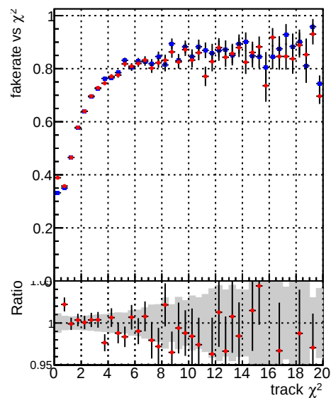
Fake rate vs. —●— DQM_TT_mkFit-DQM_original-0 —●— DQM_TT_mkFit-DQM_updated-0
