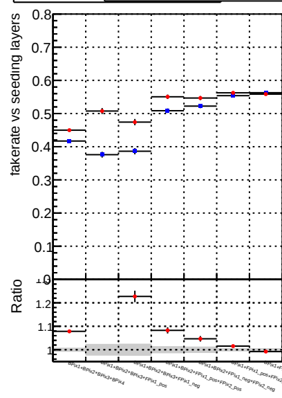
Fake rate vs. —●— DQM_TT_mkFit-DQM_original-0 —●— DQM_TT_mkFit-DQM_updated-0
