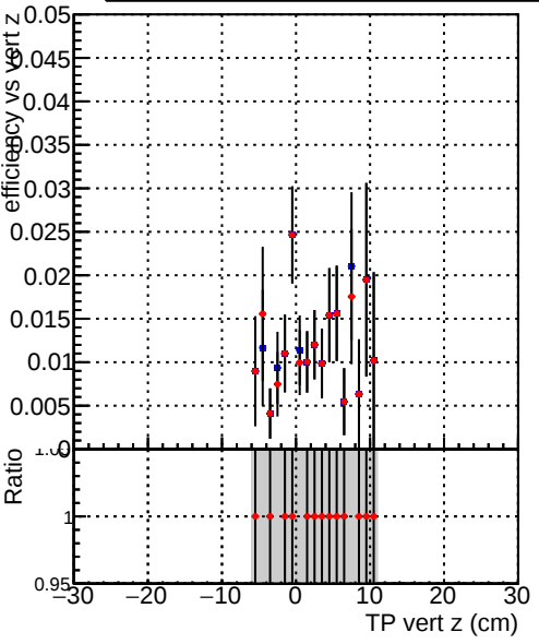
Efficiency vs TP vert z (cm) Legend: DQM_TT_mkFit-DQM_original-0 (Blue diamonds) DQM_TT_mkFit-DQM_updated-0 (Red diamonds)
