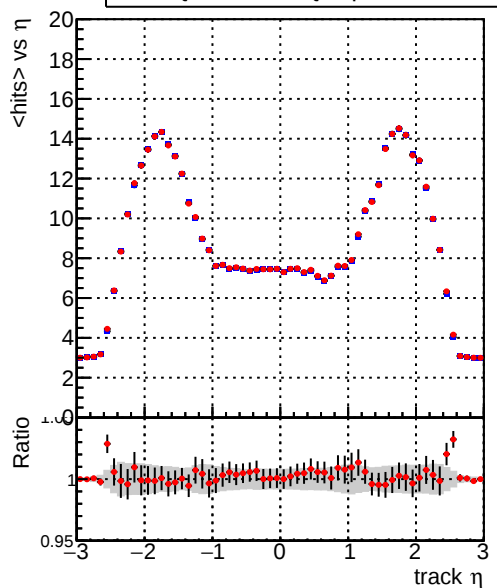
— DQM_TT_mkFit-DQM_original-0 — DQM_TT_mkFit-DQM_updated-0
