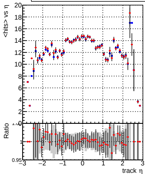
mean hits DQM_TT_mkFit-DQM_original-0 DQM_TT_mkFit-DQM_updated-0
