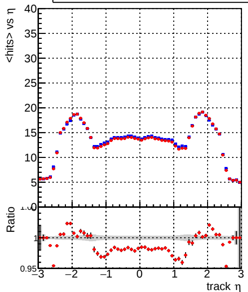
mean hits — DQM_TT_mkFit-DQM_original-0 — DQM_TT_mkFit-DQM_updated-0
