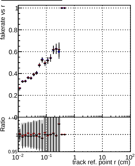
Fake rate vs verpos DOM_TT_CKF_ORIG DOM_TT_CKFandPless_ORIG DOM_TT_CKFandPless_MODIF
