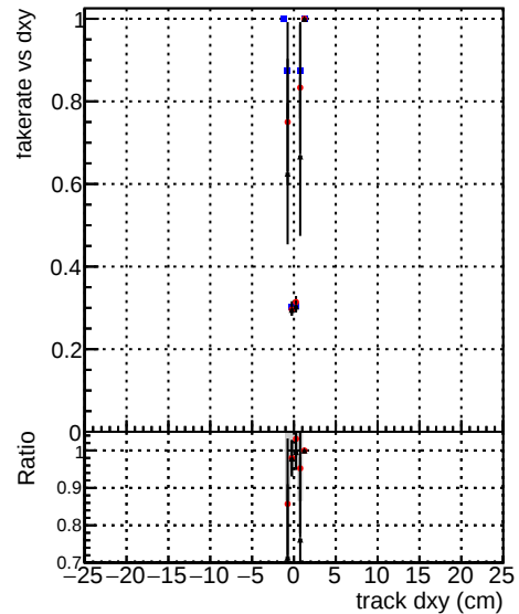
Fake rate vs d DOM TT CKF ORIG DOM TT CKFandPless ORIG DOM TT CKFandPless MODIF
