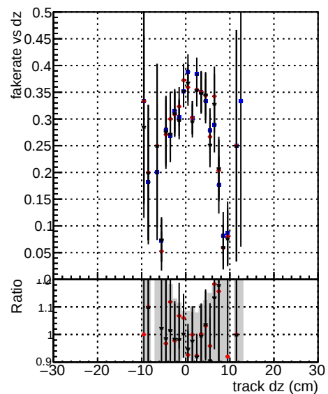
Fake rate vs d DOM TT CKF ORIG DOM TT CKFandPless ORIG DOM TT CKFandPless MODIF
