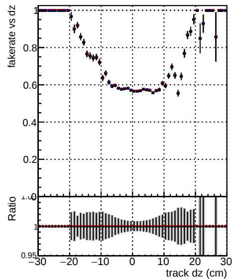
Fake rate vs dz —●— DOM TT CKF ORIG —●— DOM TT CKFandPless ORIG —●— DOM TT CKFandPless MODIF
