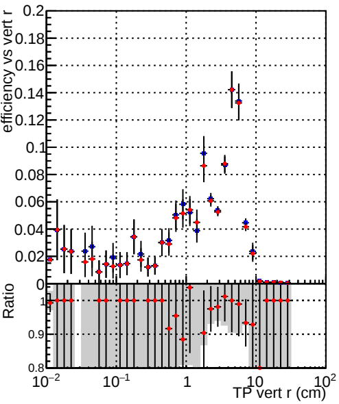
Efficiency vs TP vert r (cm) Legend: DQM_TT_MKFIT_ORIG (blue squares), DQM_TT_MKFIT_MODIF (red circles)
