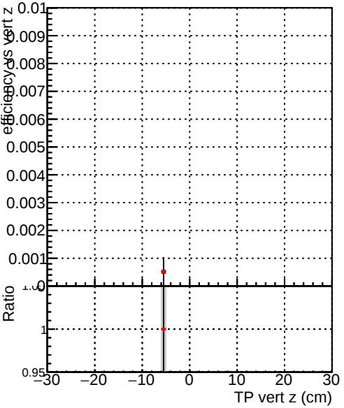
Efficiency vs. TP vert z Legend: DQM_TT_MKFIT_ORIG DQM_TT_MKFIT_MODIF
