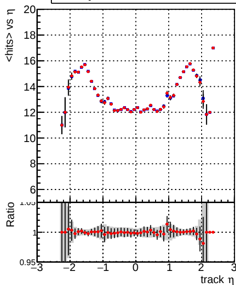
mean hits vs \eta Legend: DQM_TT_MKFIT_ORIG (blue line with markers), DQM_TT_MKFIT_MODIF (red line with markers)
