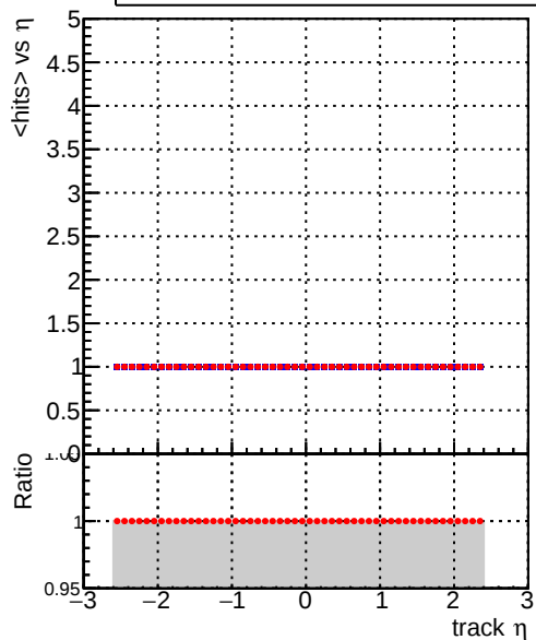
mean hits — DQM_TT_MKFIT_ORIG — DQM_TT_MKFIT_MODIF
