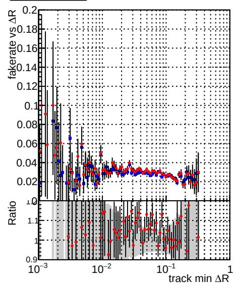
—■— DQM_TT_MKFIT_ORIG —●— DQM_TT_MKFIT_MODIF
