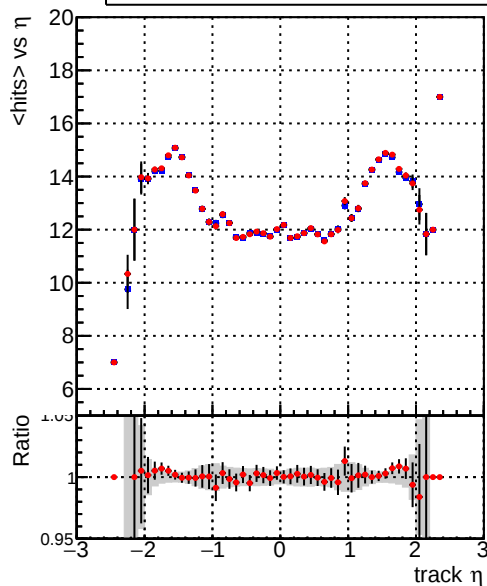
mean hits vs \eta — DQM_TT_MKFIT_ORIG — DQM_TT_MKFIT_MODIF
