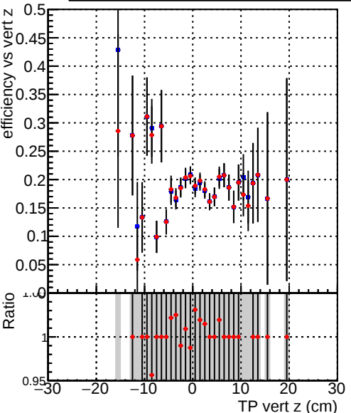
Efficiency vs vertpos Legend: DQM_TT_MKFIT_ORIG (blue squares), DQM_TT_MKFIT_MODIF (red circles)
