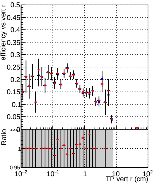
Efficiency vs vertpos Legend: DQM_TT_MKFIT_ORIG (blue squares), DQM_TT_MKFIT_MODIF (red circles)
