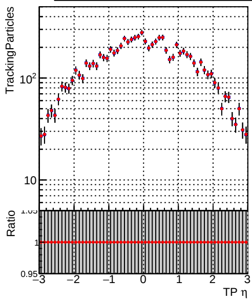
N of simulated tracks vs TP \eta Legend: DQM_TT_MKFIT_ORIG (blue line with dots), DQM_TT_MKFIT_MODIF (red line with dots)
